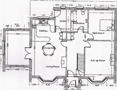
GROUND FLOOR PLAN 125.3 SQ METRES
